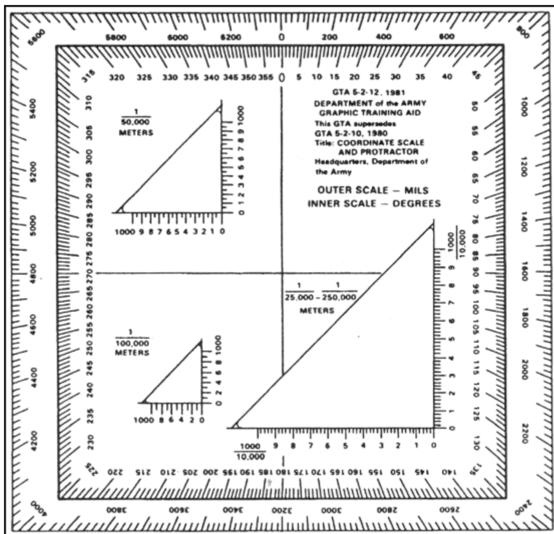
Figure 4-14. Coordinate scales.
