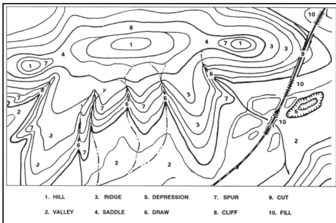
Figure 10-26. Terrain features.
