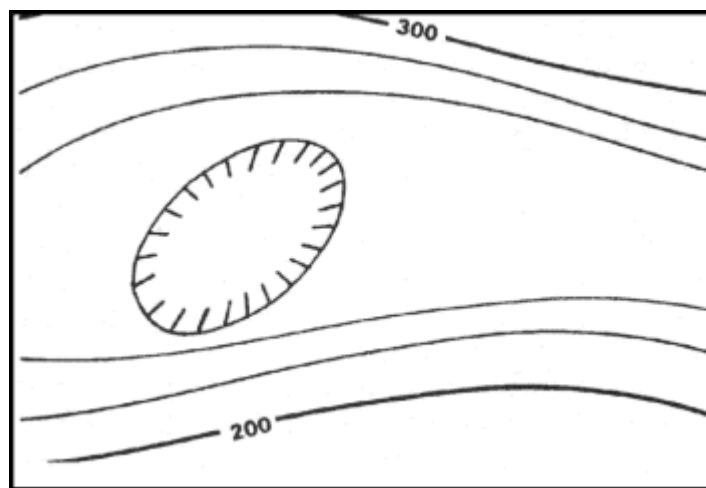
Figure 10-5. Depression.
