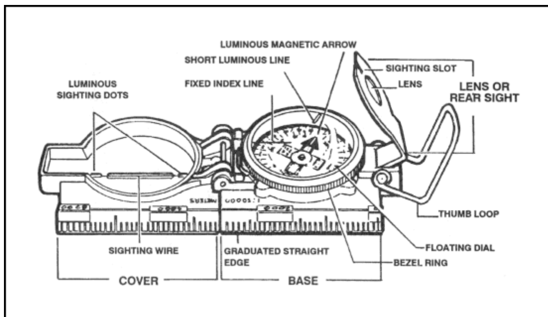
Figure 9-1. Lensatic compass.
