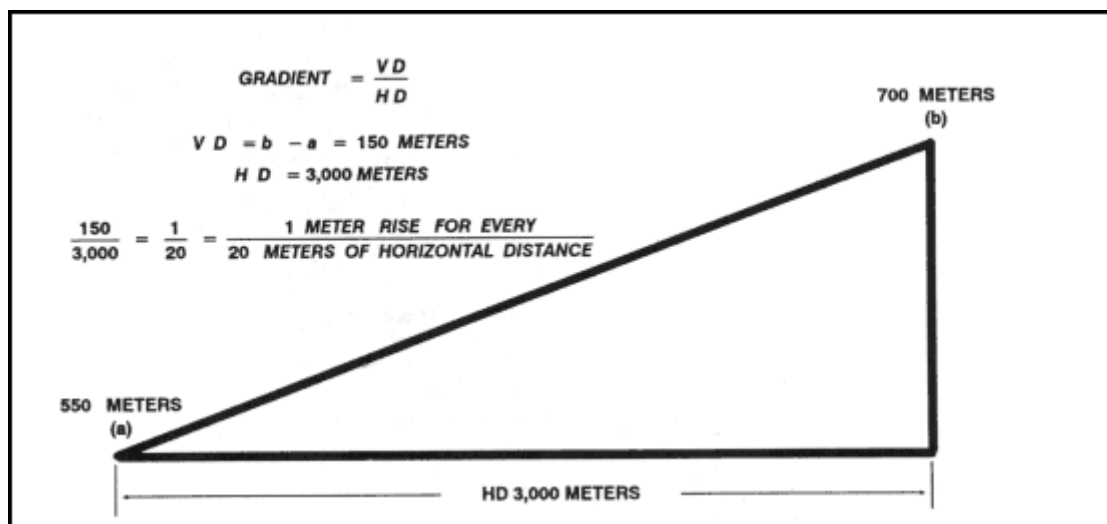
Figure 10-15. Gradient.
