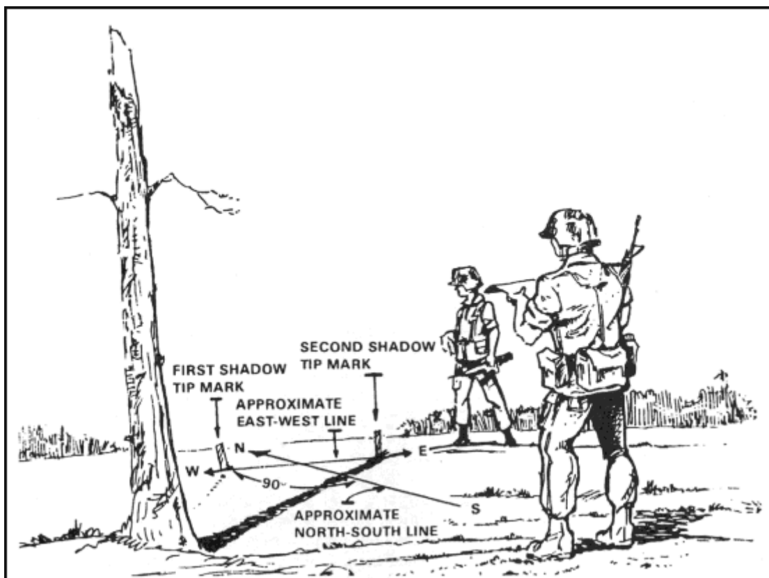
Figure 11-6. Field-expedient method.
