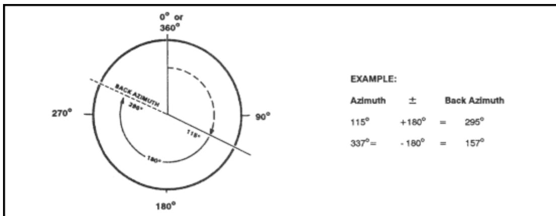
Figure 6-3. Back azimuth.
