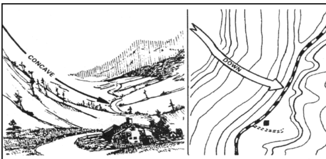
Figure 10-8. Concave slope.
